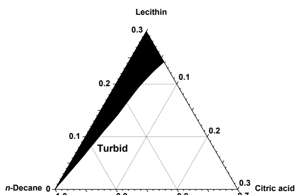
Fig. 1 Partial phase diagram of citric acid/lecithin/ n -decane system in the dilute region at 25°C. The phase states were identified by visual observation through crossed polarizers or SAXS analysis.
