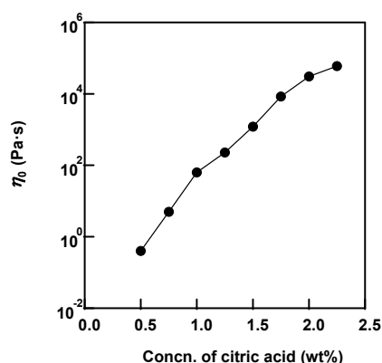
Fig. 2 Zero-shear viscosity ( \eta_0 ) of citric acid/lecithin/ n -decane systems as a function of citric acid concentration at 25°C. Lecithin concentration was fixed at 10 wt%.
