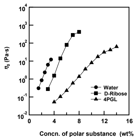
Fig. 3 Zero-shear viscosity ( \eta_0 ) of polar substance/lecithin/IPM/TES systems as a function of polar substances concentrations at 32°C. Lecithin concentration was fixed at 30 wt%.
