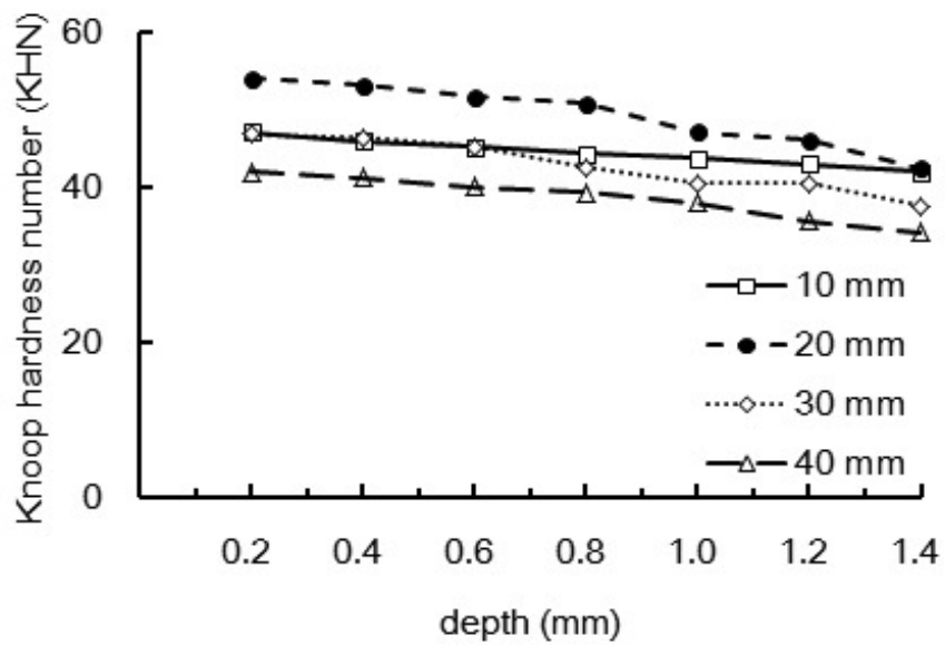
Fig. 2. Knoop hardness number (KHN) values of the composite material Distance from the material surface; 0.2-1.4 mm
